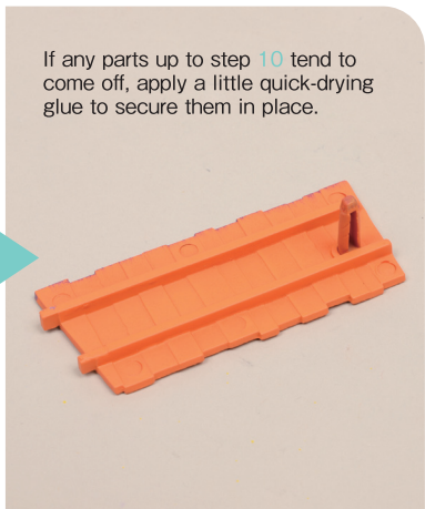
Fit the 7 Bottom Stake to the underside of the 8 Jetty by matching the shape of its protrusion with the hole in the Jetty and insert it.
